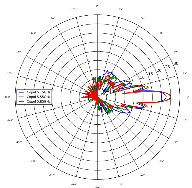
Elevation, Vertical
