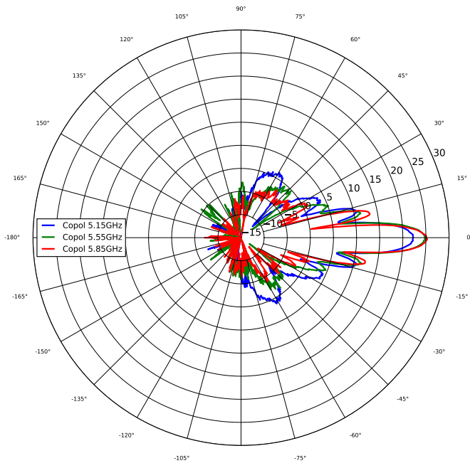
Azimuth, Horizontal
