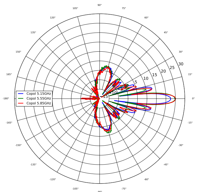
Azimuth, Vertical
